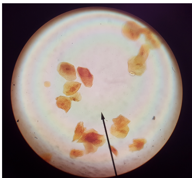
Cheek Cell (400X)
