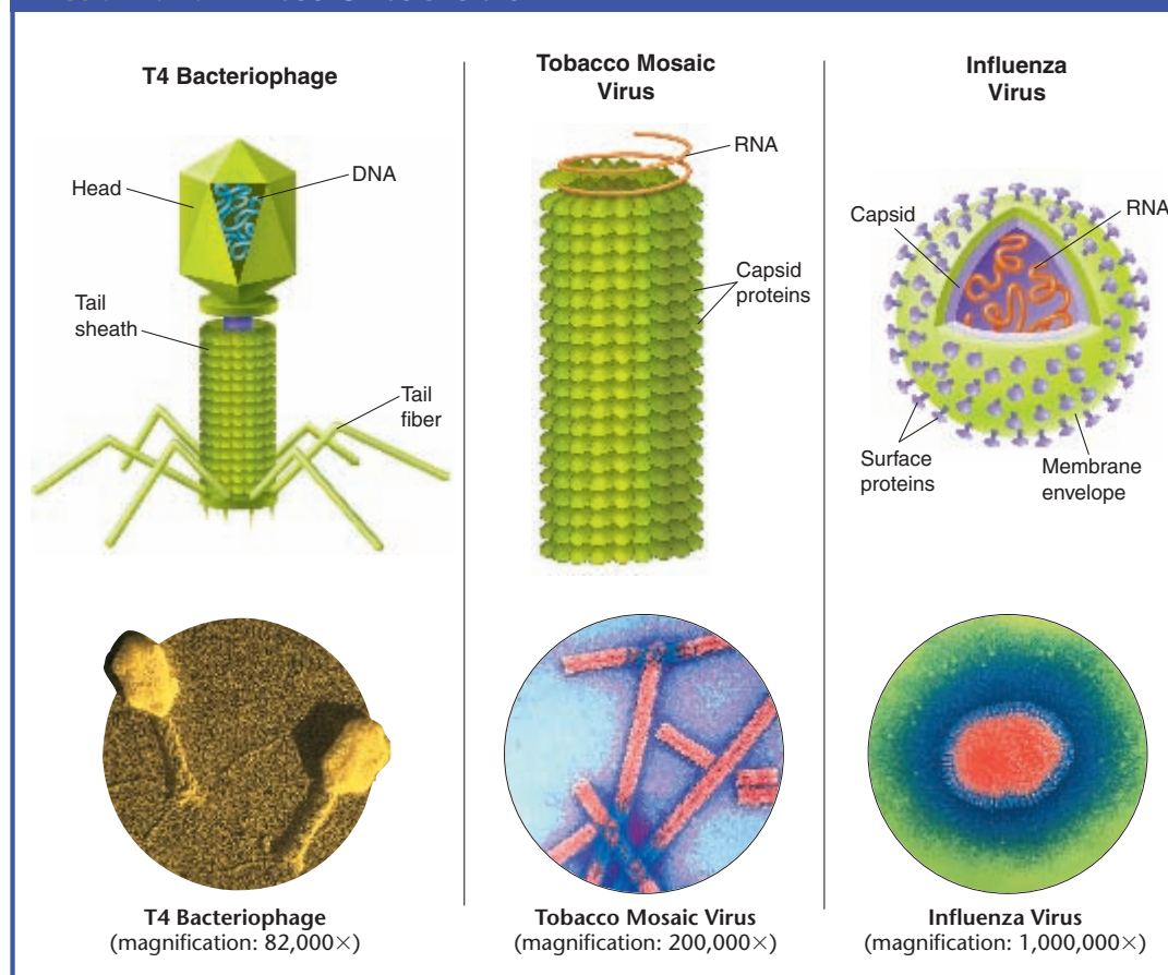
FIGURE 19-9 VIRUS STRUCTURES
